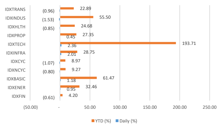
Figure 2. Sectors Movement
